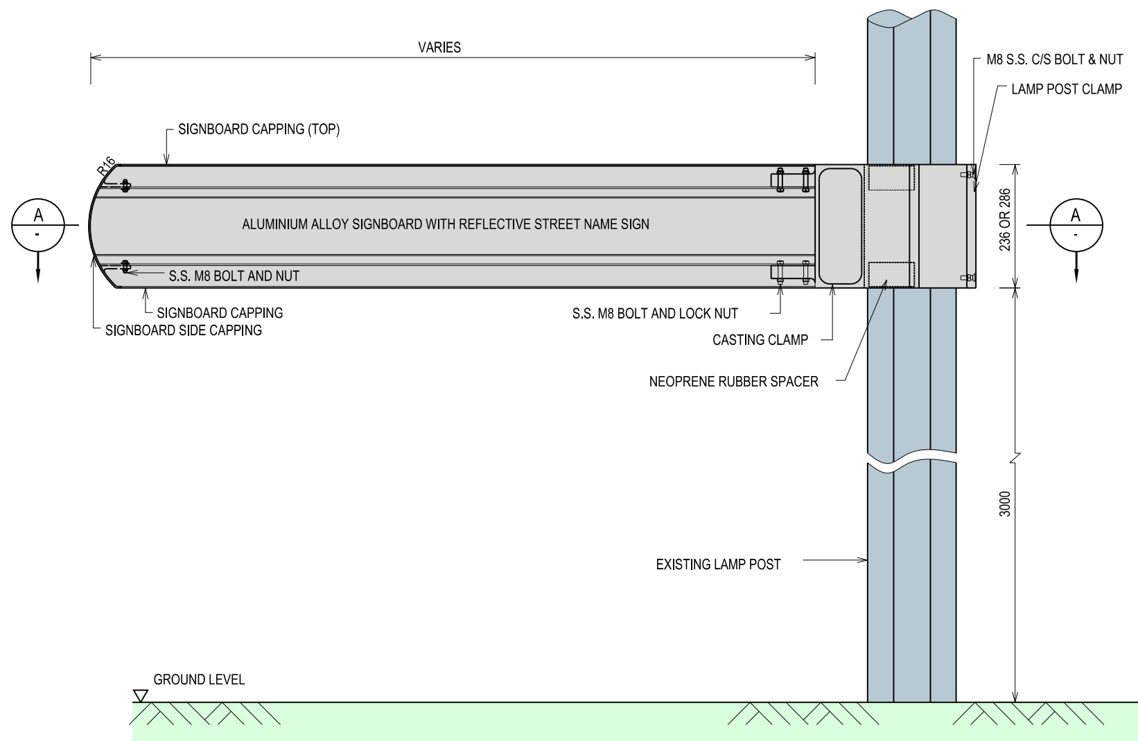
ELEVATION SCALE 1:10
