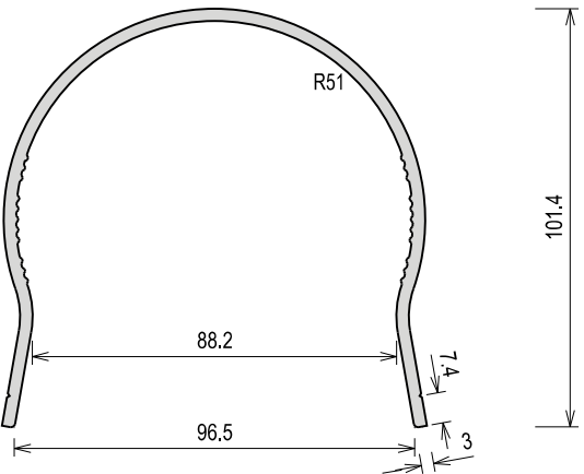
ALUMINIUM SIGN HOLDER SCALE 1:2
