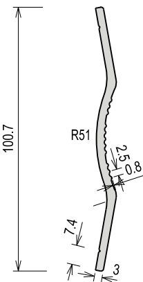
ALUMINIUM SIGN HOLDER SCALE 1:2
