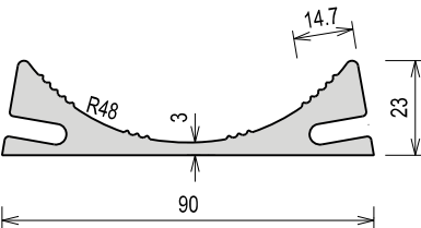
SIGN SUPPORTER SCALE 1:2
