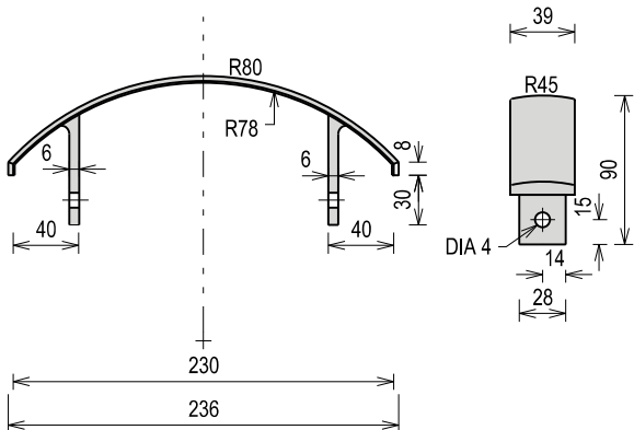
CASTING SIDE CAPPING (C4) SCALE 1:5
