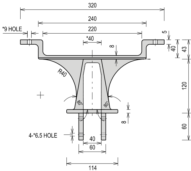
CASTING TOP HOLDER (C1) SCALE 1:5
