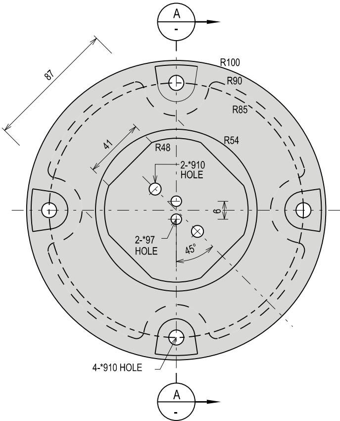
CASTING CLAMP (C2,C3) FOR C2 H=236, FOR C3 H=286 SCALE 1:5
