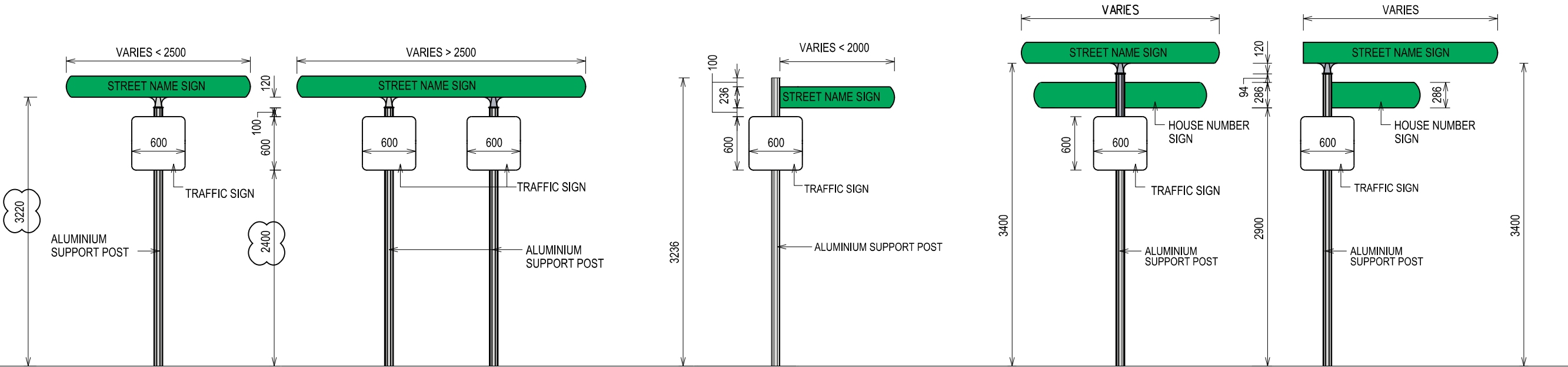
SNS-S1 SCALE 1:50
