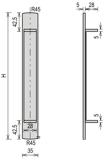
CASTING SIDE CAPPING (C7,C8) FOR C7 H=236, FOR C8 H=286 SCALE 1:5
