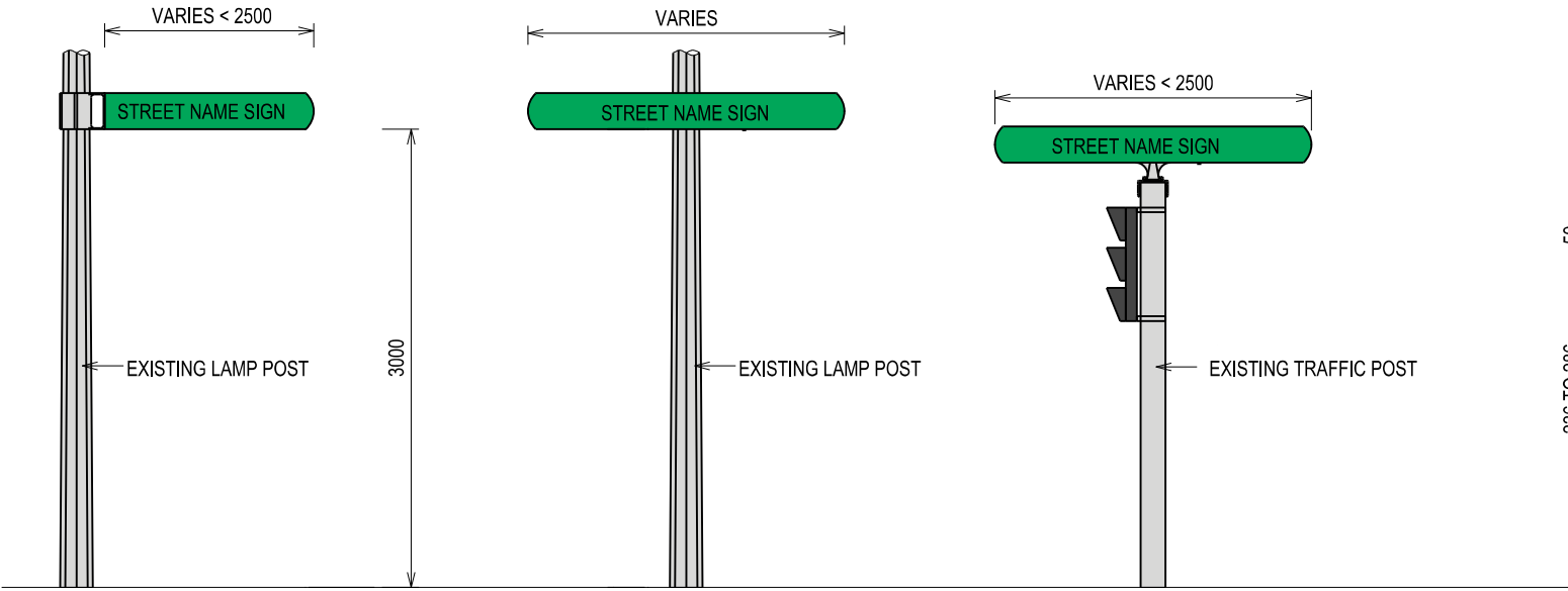
SNS-L1 SCALE 1:50
