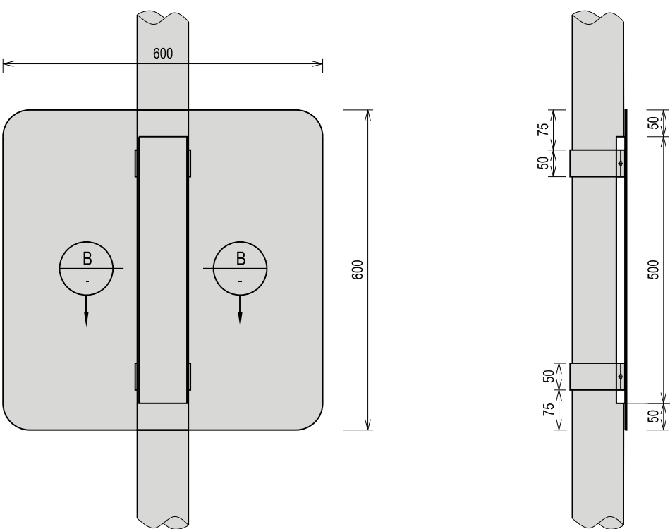
TRAFFIC SIGN ON SUPPORT POST SINGLE SIDE TYPE SCALE 1:10
