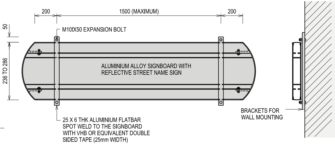
SNS-W1 SCALE 1:20
