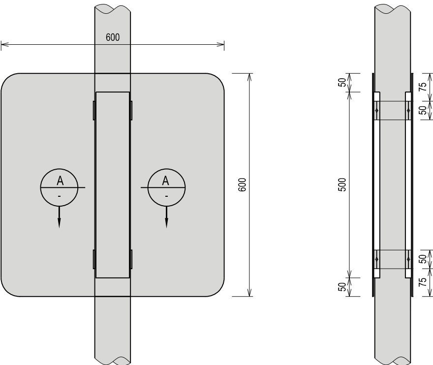
TRAFFIC SIGN ON SUPPORT POST DOUBLE SIDE TYPE SCALE 1:10
