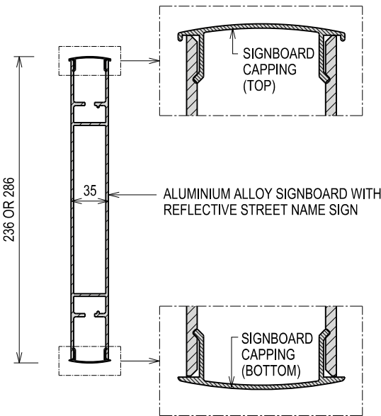
TYPICAL SIGNBOARD WITH CAPPINGS SCALE 1:5
