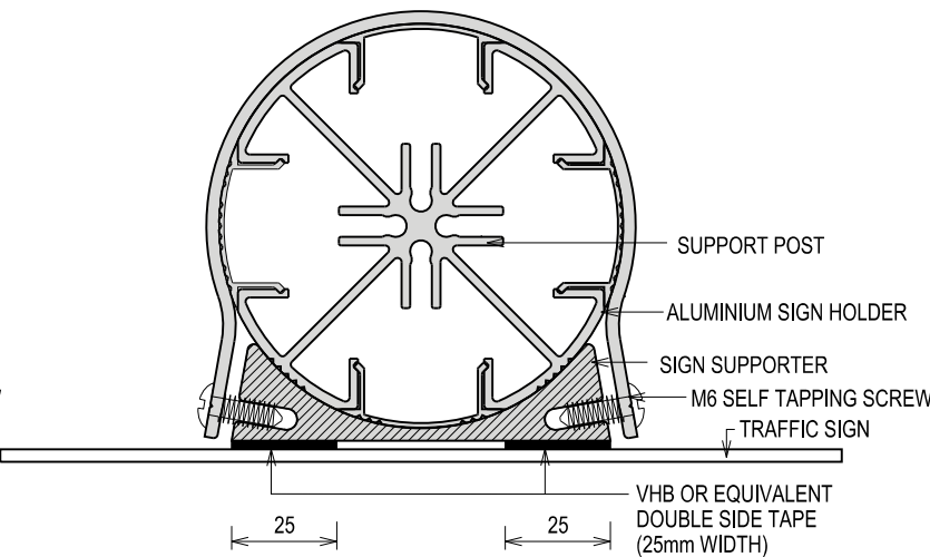
SECTION B-B SCALE 1:2
